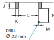
DROP-IN FRAME
